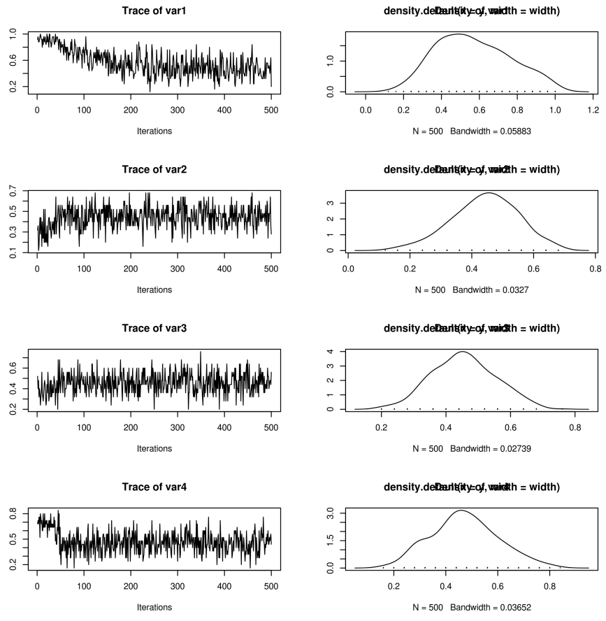
Figure 1: Metropolis acceptance trace plots.
